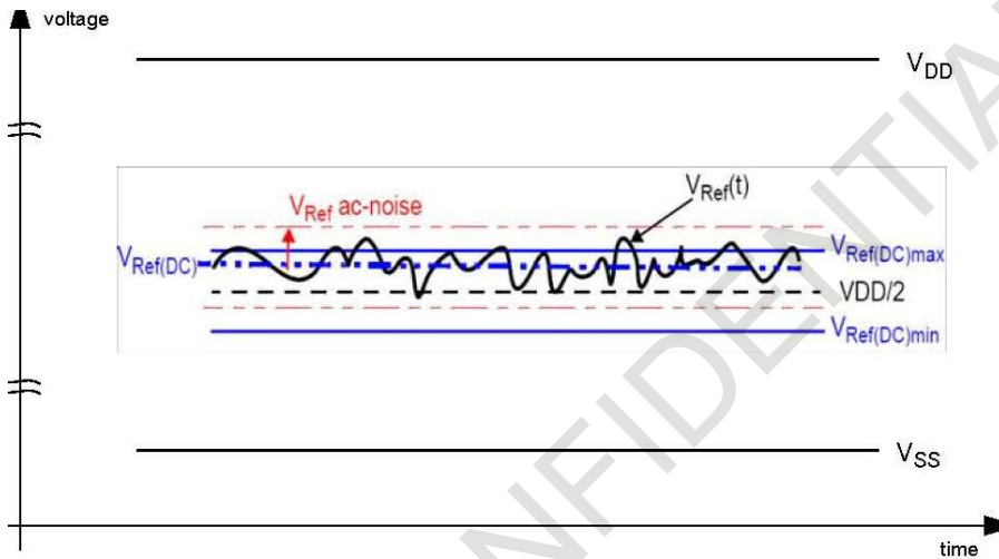
Illustration of V_{REF(DC)} tolerance and V_{REF} \text{ AC-noise} limits
